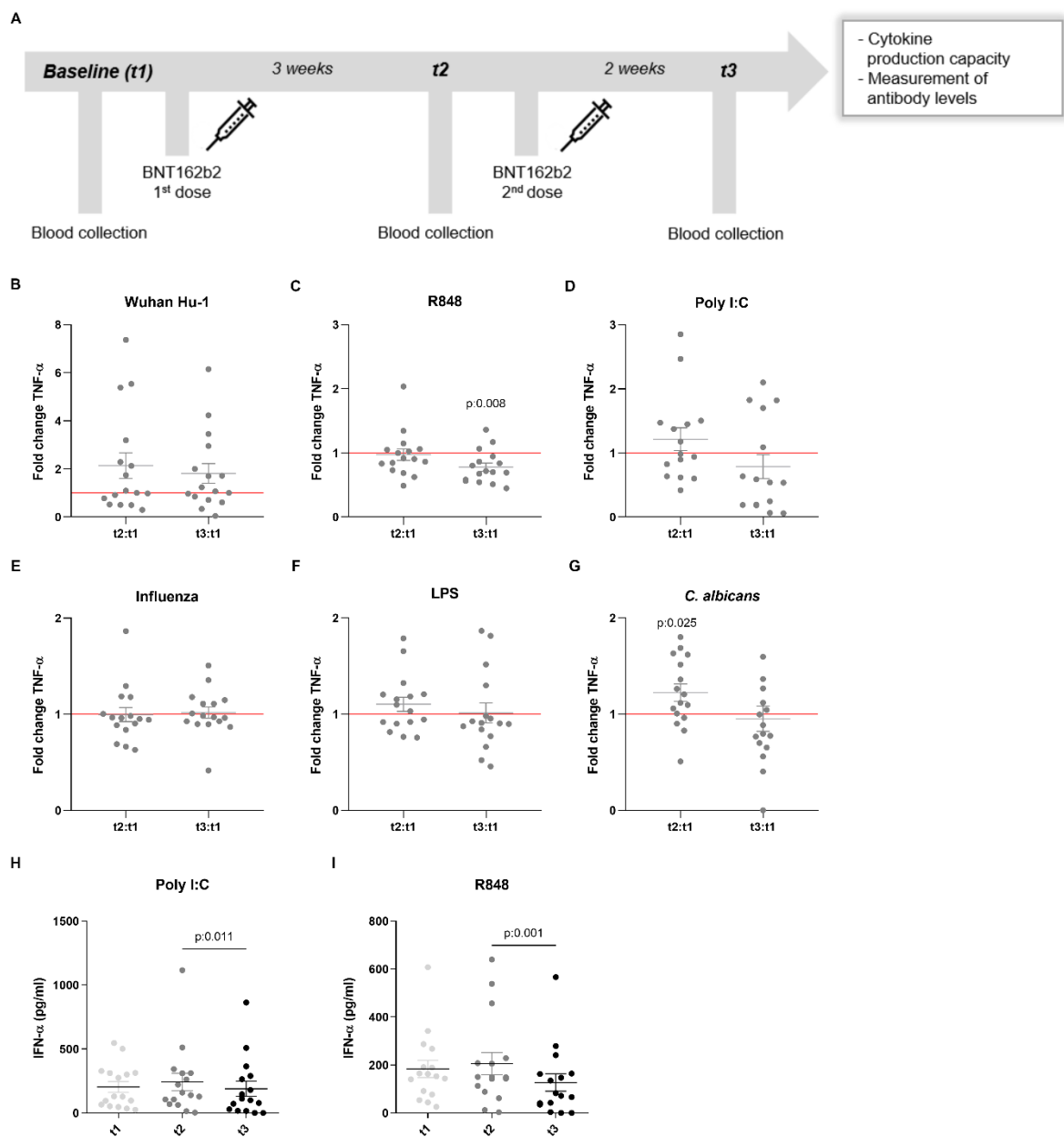
265 Figure 1. TNF-α and IFN-α production in response to heterologous stimuli in PBMCs isolated 266 from vaccinated subjects. (A) Description of the study: vaccination and blood collection days. 267 (B-G) Fold change values of TNF-α production are calculated individually for each subject by 268 division of t2:t1 and t3:t1. Data are presented as fold changes ± SEM (n=15-16) and analysed 269 by Wilcoxon's matched-pairs signed-rank test comparing each ratio to t1=1 (red line). (H-I) 270 IFN-α production (pg/ml) at t1, t2 and t3. Data are presented as cytokine concentration ± SEM 271 (n=15-16) and analysed by Wilcoxon's matched-pairs signed-rank test.
